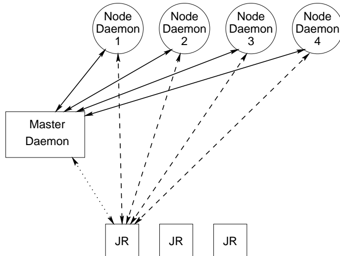
Figure 1: General cluster architecture. The master daemon handles resource management with the job representative processes (JR), and controls the node daemons.
