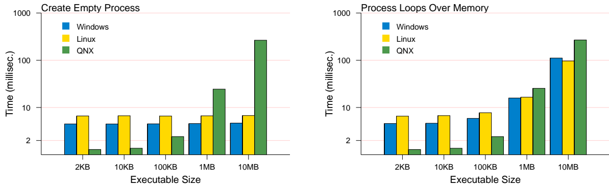
Figure 2: Process Creation and Termination Times.
