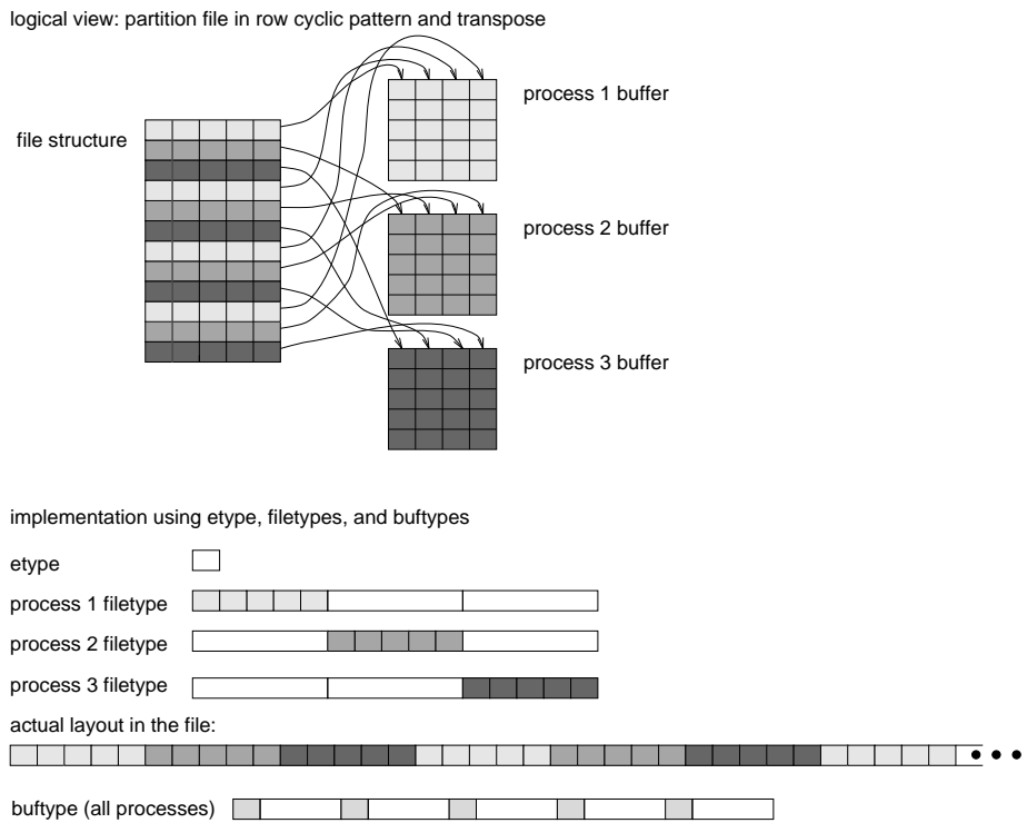
Figure 3 Transposing and partitioning a 2-D matrix
