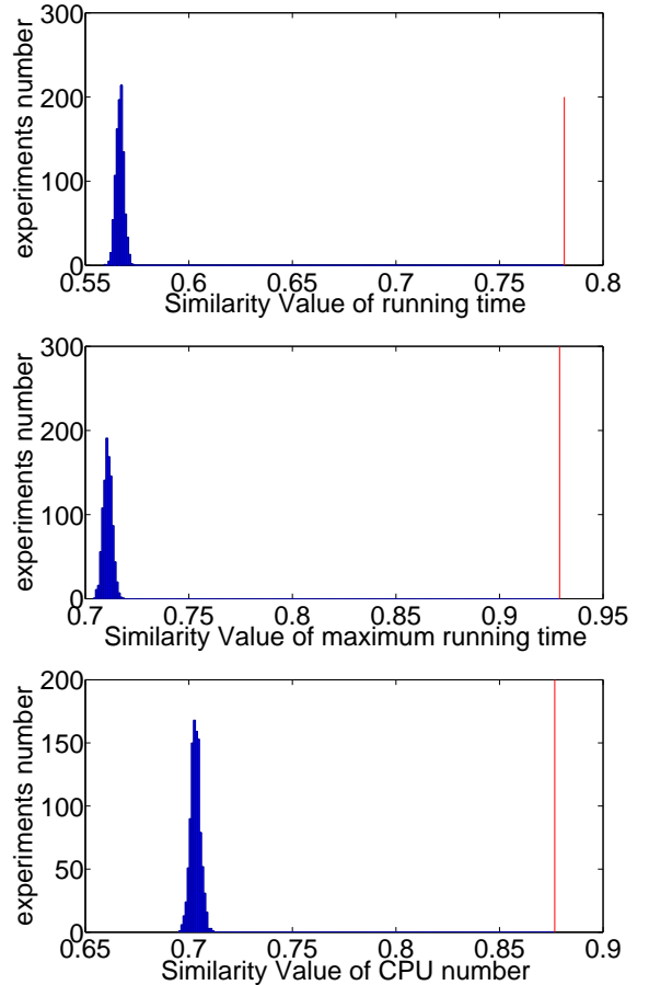
Figure 2: Comparison of the similarity between jobs in the same session as computed from the SDSC-SP2 log (vertical line), and the distribution of similarity levels that are seen when the jobs are randomized.
